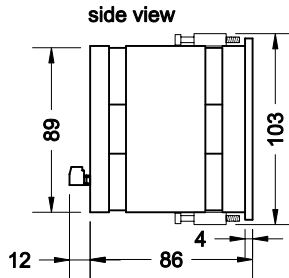
case dimensions
